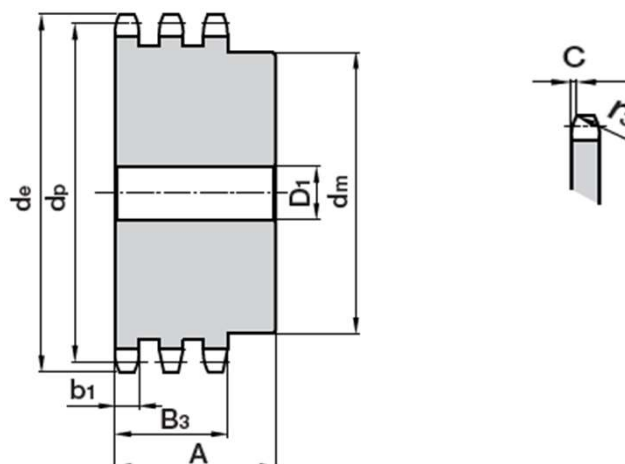
3/8" x 7/32" TRIPLEX
