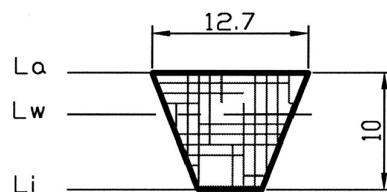
XPA/SPA
