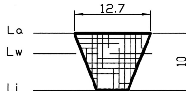
XPA/SPA
