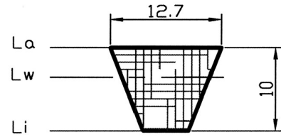
XPA/SPA
