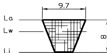
XPZ/SPZ
