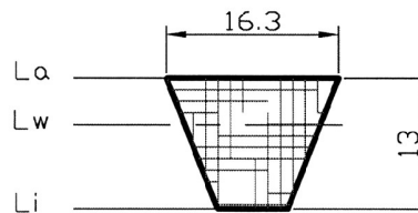
XPB/SPB
